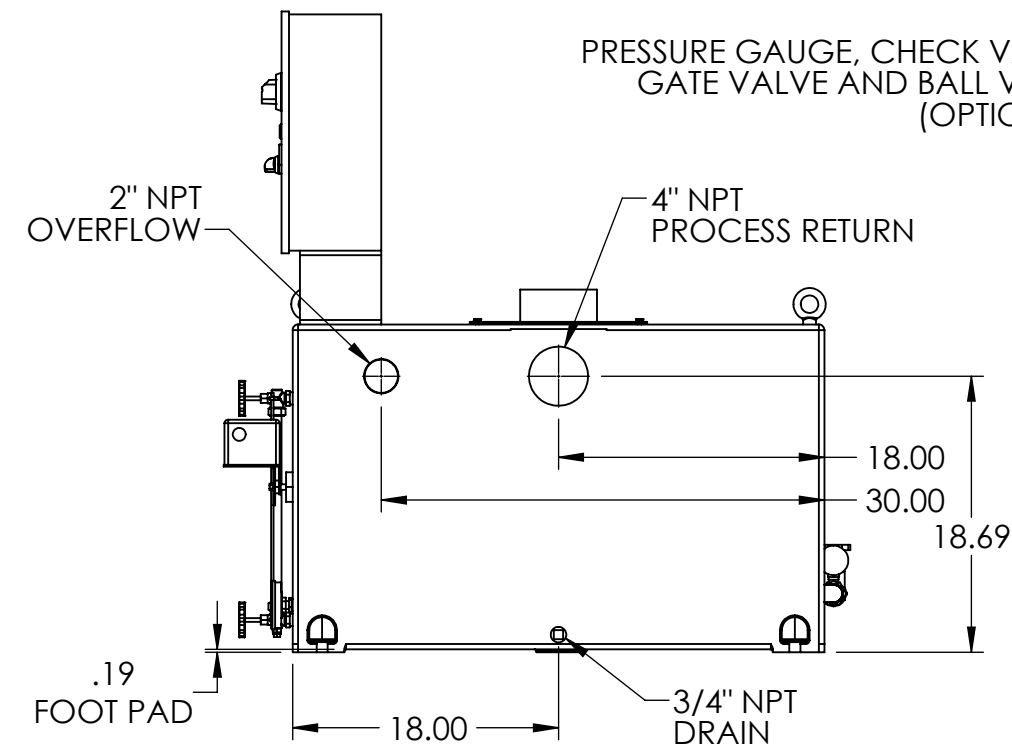
BACK VIEW
